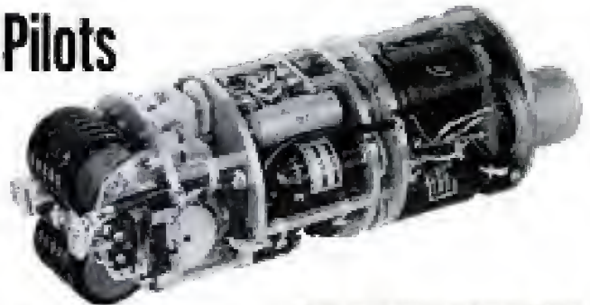
Ford Instrument Company photo Counters at left end of indicator unit, above, tell pilot the aircraft's present latitude and longitude
